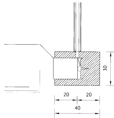
Detail aansluiting lamp, fitting en snoer Detail connection lamp, lamp holder and flex
